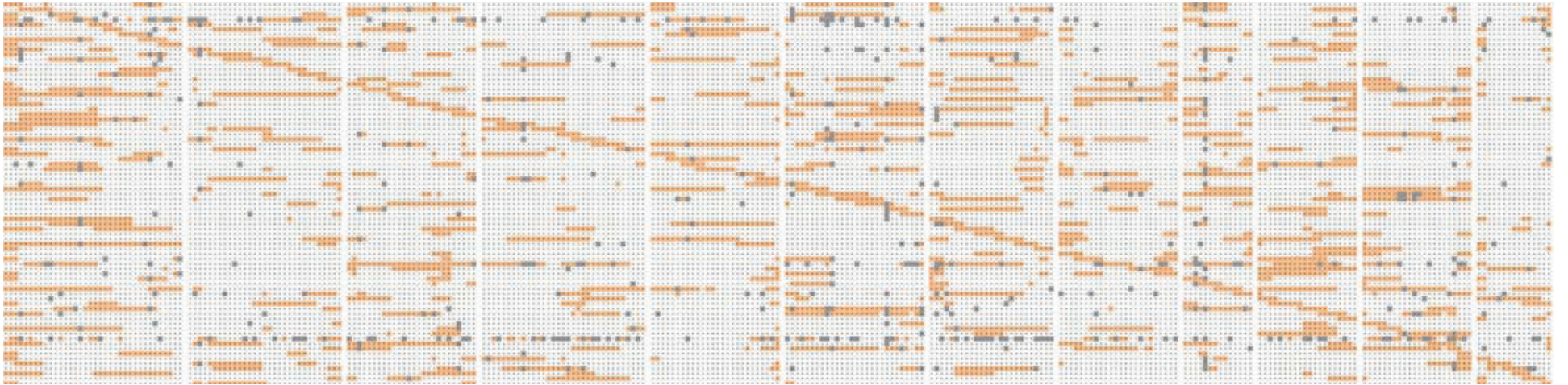
Supplementary Fig. S3 A graphical genotype of 77 BC2 lines using RiceOPA6.0 generated during the process of CSSL development.
