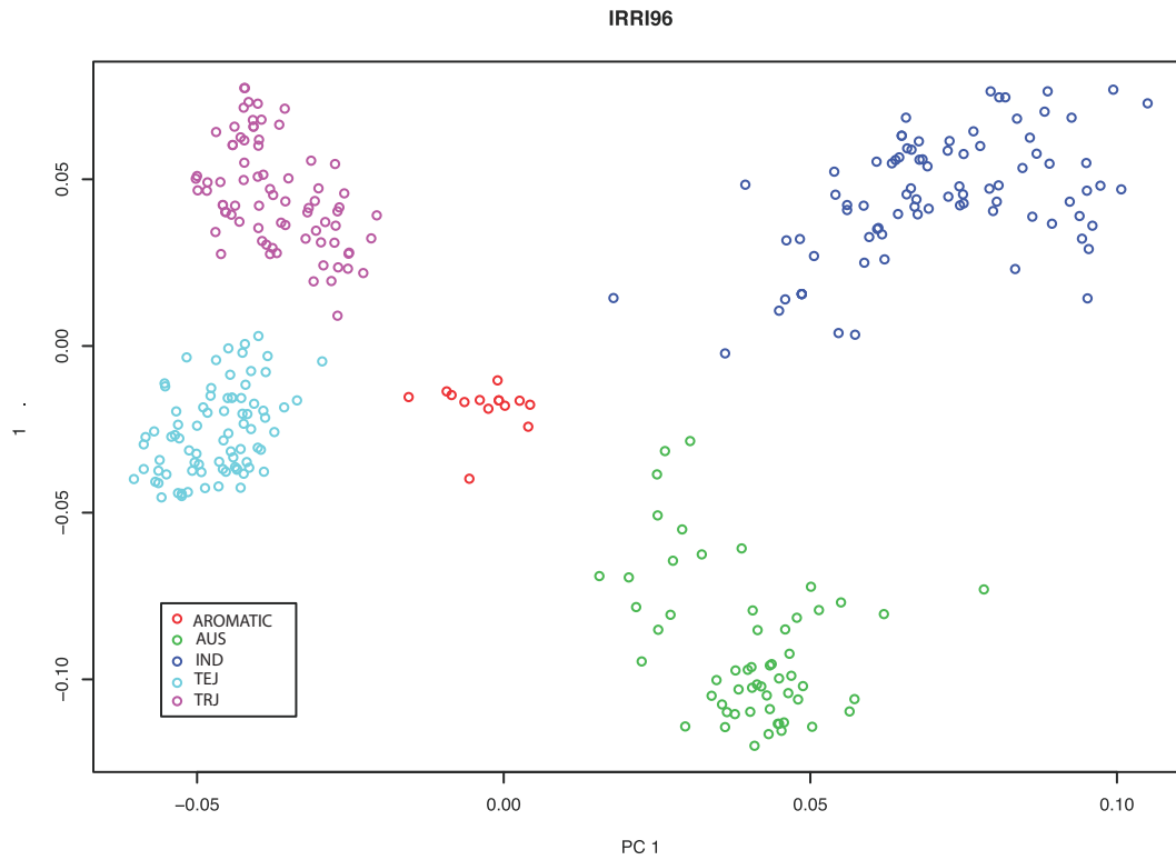
Supplementary Fig. S1 A principal coordinate analysis from the 96 SNPs of RiceOPA1.0 showing clear separation of all five O. sativa population subgroups across a set of diverse germplasm.
