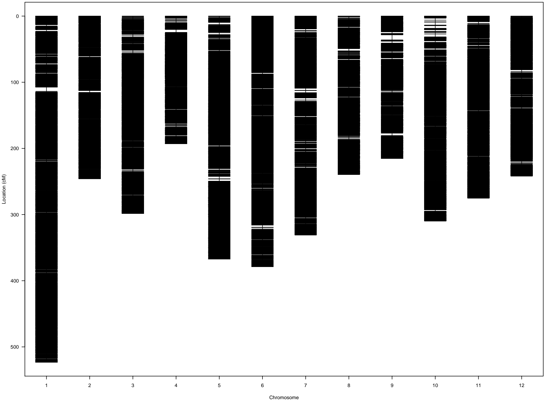
Genetic map
